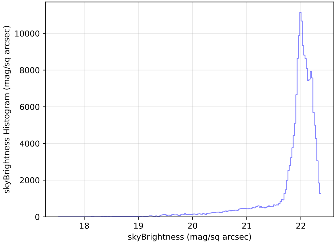
internal_u_expt30_nscale1.5v3.4_10yrs All sky g band: skyBrightness Histogram
