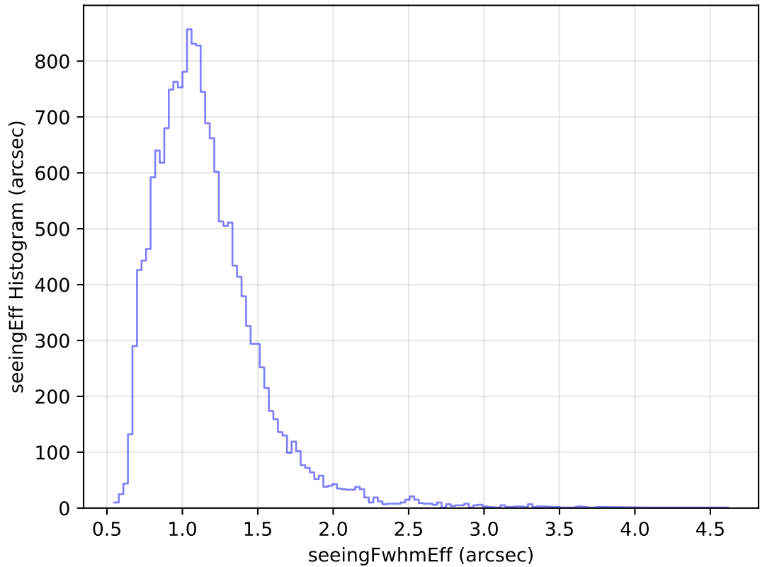
internal_u_expt30_nscale1.5v3.4_10yrs Yr 1 u band: seeingEff Histogram
