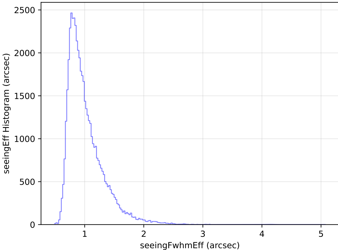
internal_u_expt30_nscale1.5v3.4_10yrs Yr 1 r band: seeingEff Histogram
