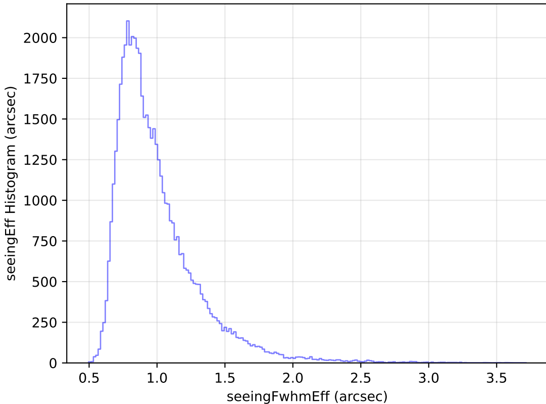
internal_u_expt30_nscale1.5v3.4_10yrs Yr 1 i band: seeingEff Histogram
