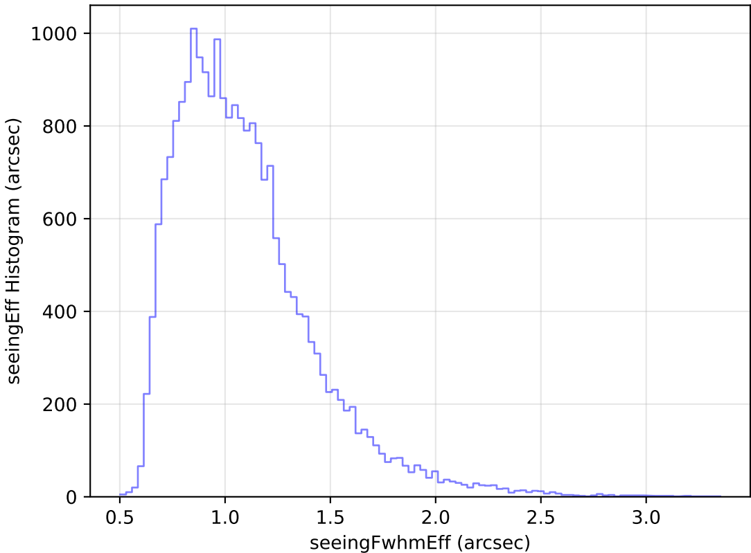
internal_u_expt30_nscale1.5v3.4_10yrs Yr 1 g band: seeingEff Histogram
