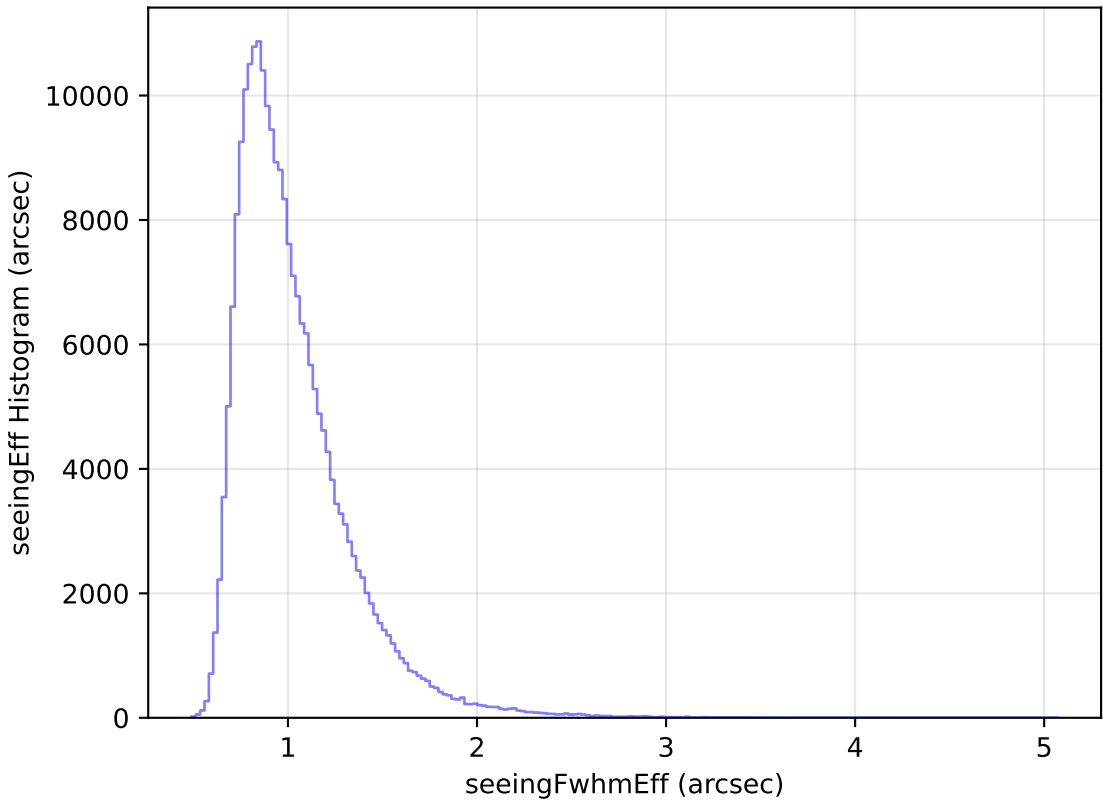
internal_u_expt30_nscale1.5v3.4_10yrs Yr 1 all bands: seeingEff Histogram
