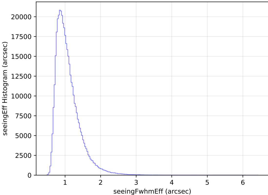
internal_u_expt30_nscale1.5v3.4_10yrs WFD z band: seeingEff Histogram
