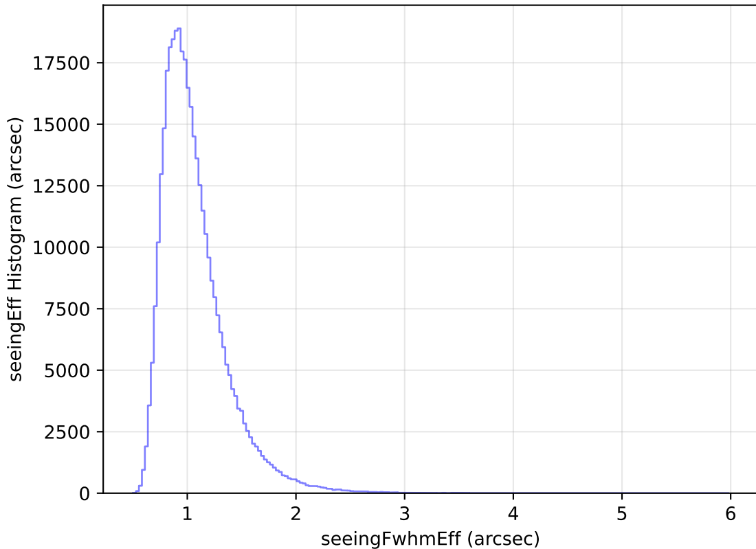
internal_u_expt30_nscale1.5v3.4_10yrs WFD y band: seeingEff Histogram
