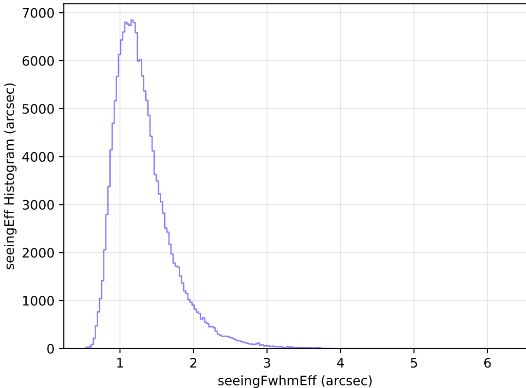
internal_u_expt30_nscale1.5v3.4_10yrs WFD u band: seeingEff Histogram
