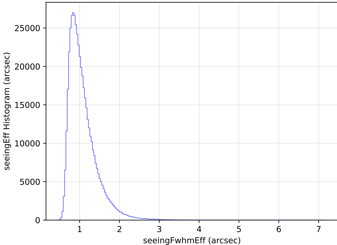
internal_u_expt30_nscale1.5v3.4_10yrs WFD i band: seeingEff Histogram
