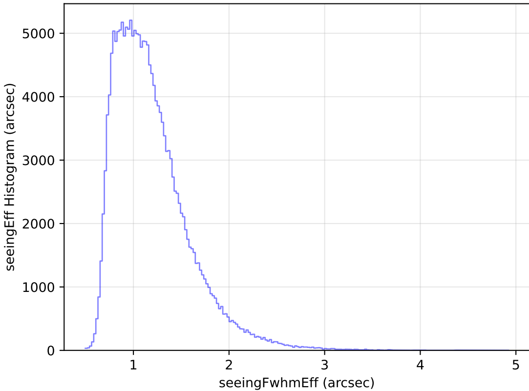
internal_u_expt30_nscale1.5v3.4_10yrs WFD g band: seeingEff Histogram
