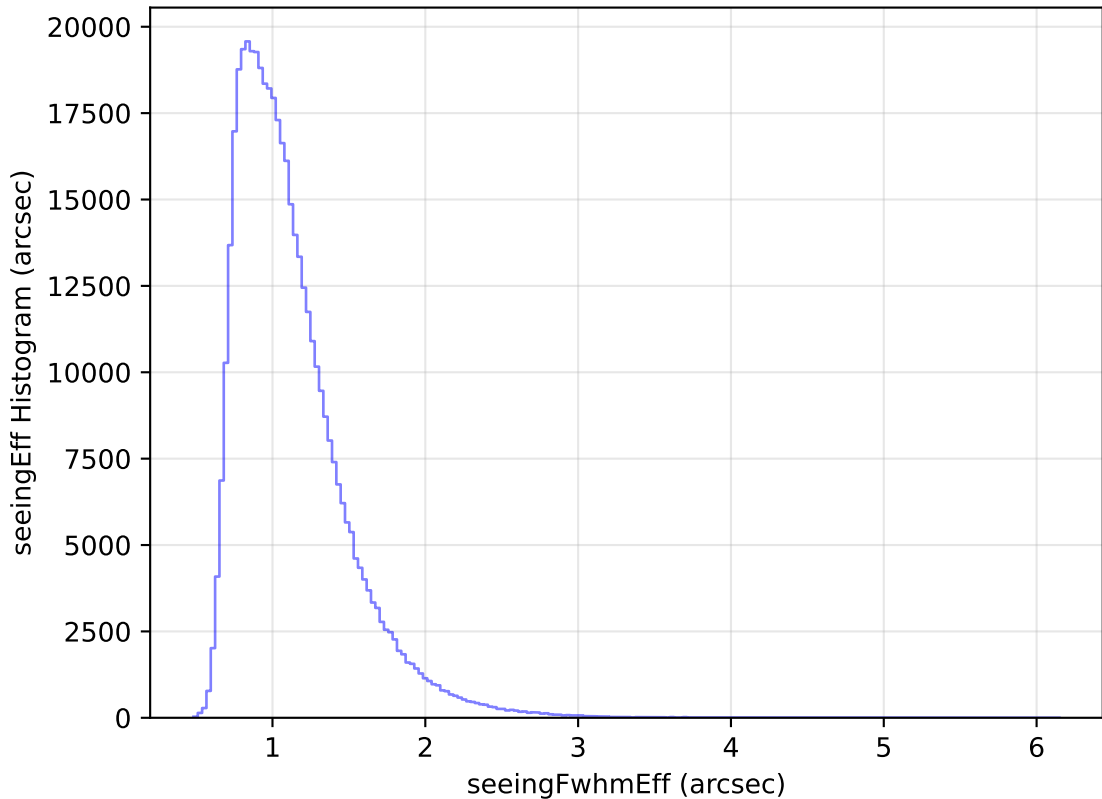
internal_u_expt30_nscale1.5v3.4_10yrs All sky r band: seeingEff Histogram
