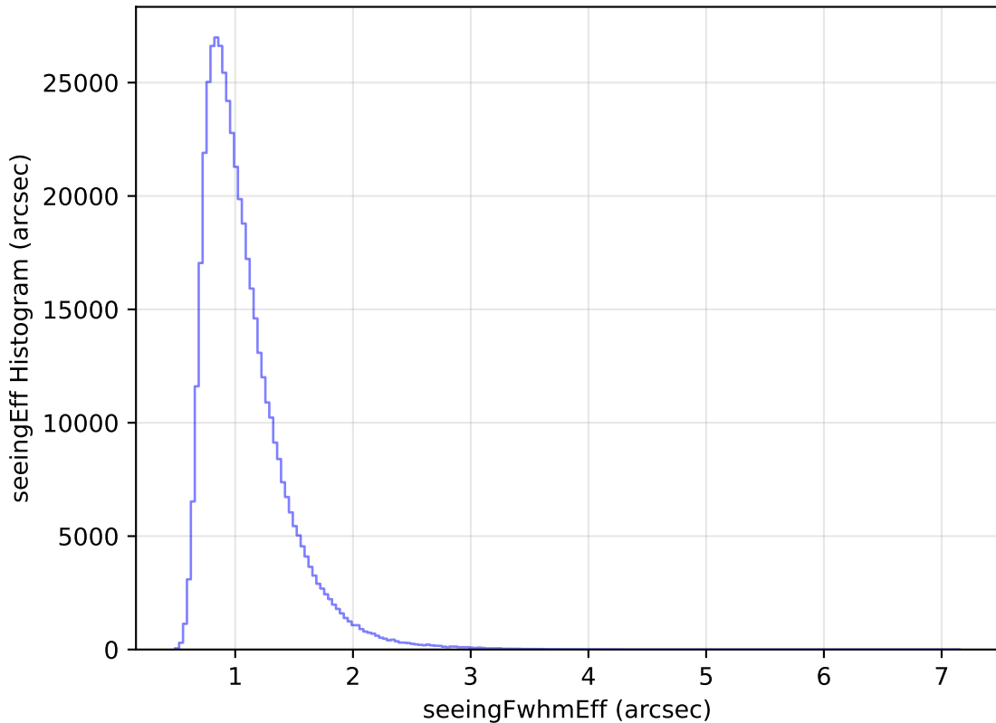
internal_u_expt30_nscale1.5v3.4_10yrs All sky i band: seeingEff Histogram
