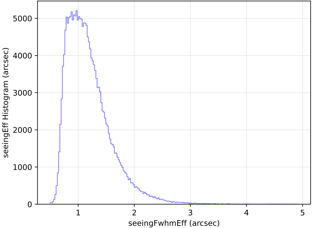
internal_u_expt30_nscale1.5v3.4_10yrs All sky g band: seeingEff Histogram
