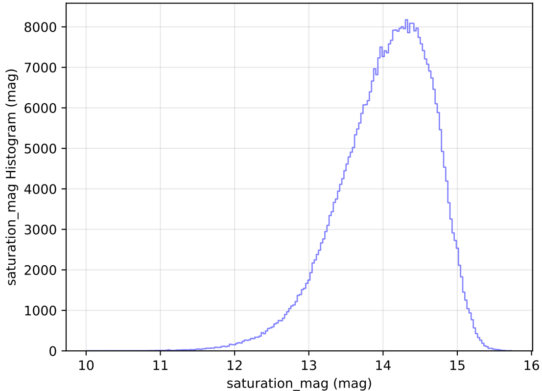
internal_u_expt30_nscale1.5v3.4_10yrs WFD z band: saturation_mag Histogram
