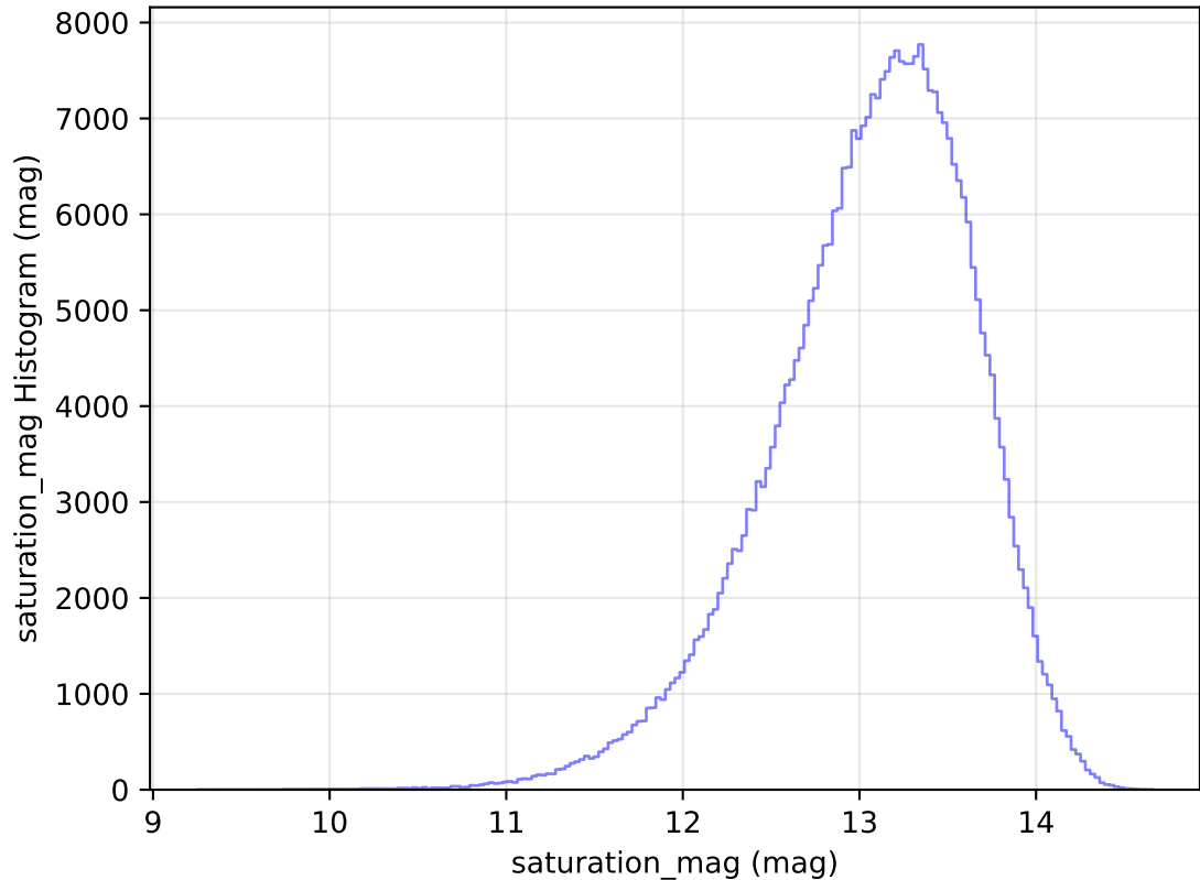
internal_u_expt30_nscale1.5v3.4_10yrs WFD y band: saturation_mag Histogram
