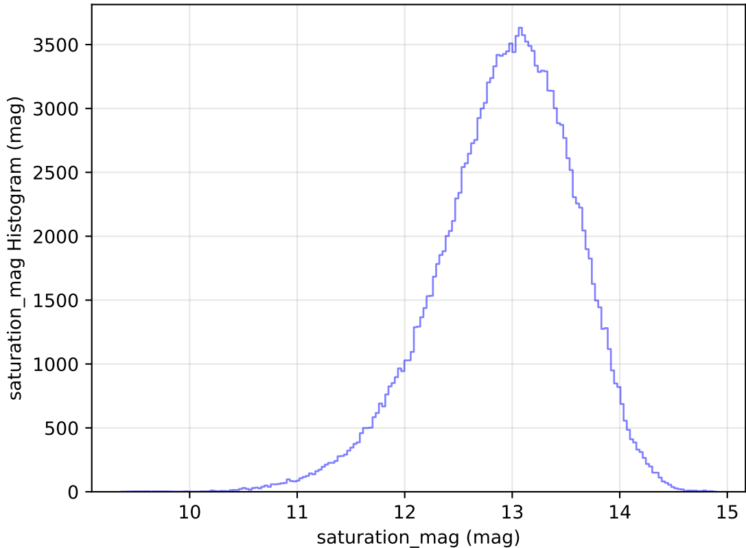
internal_u_expt30_nscale1.5v3.4_10yrs WFD u band: saturation_mag Histogram
