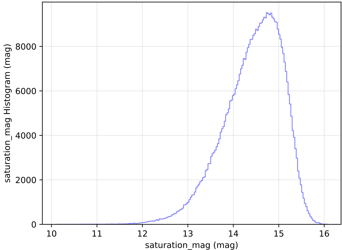
internal_u_expt30_nscale1.5v3.4_10yrs WFD i band: saturation_mag Histogram
