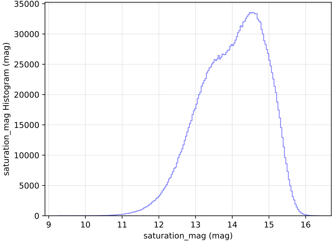
internal_u_expt30_nscale1.5v3.4_10yrs WFD all bands: saturation_mag Histogram
