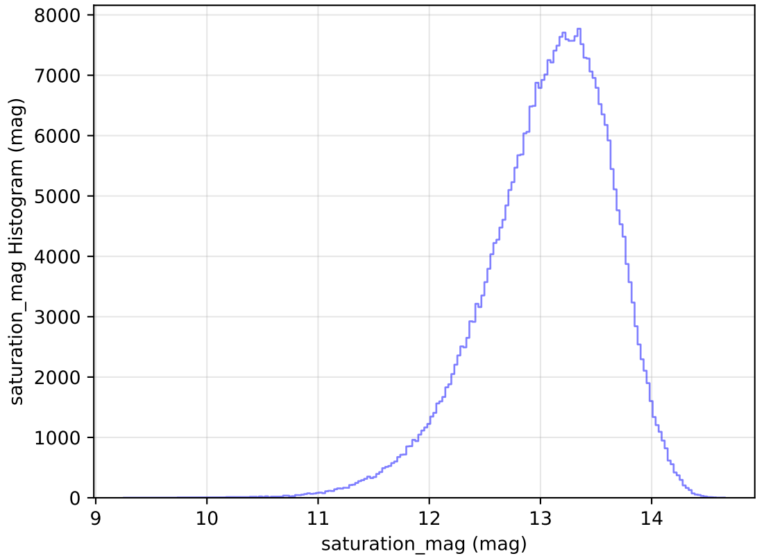
internal_u_expt30_nscale1.5v3.4_10yrs All sky y band: saturation_mag Histogram
