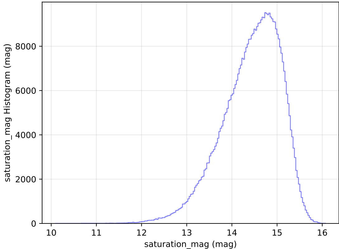
internal_u_expt30_nscale1.5v3.4_10yrs All sky i band: saturation_mag Histogram
