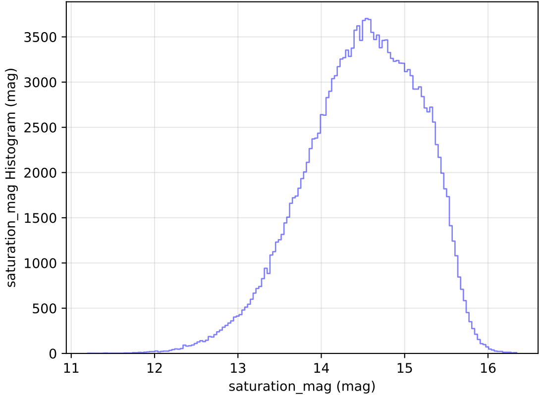
internal_u_expt30_nscale1.5v3.4_10yrs All sky g band: saturation_mag Histogram
