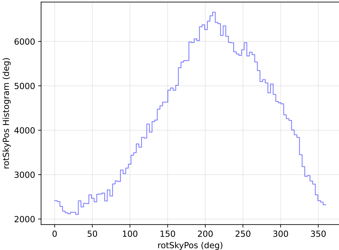
internal_u_expt30_nscale1.5v3.4_10yrs WFD z band: rotSkyPos Histogram
