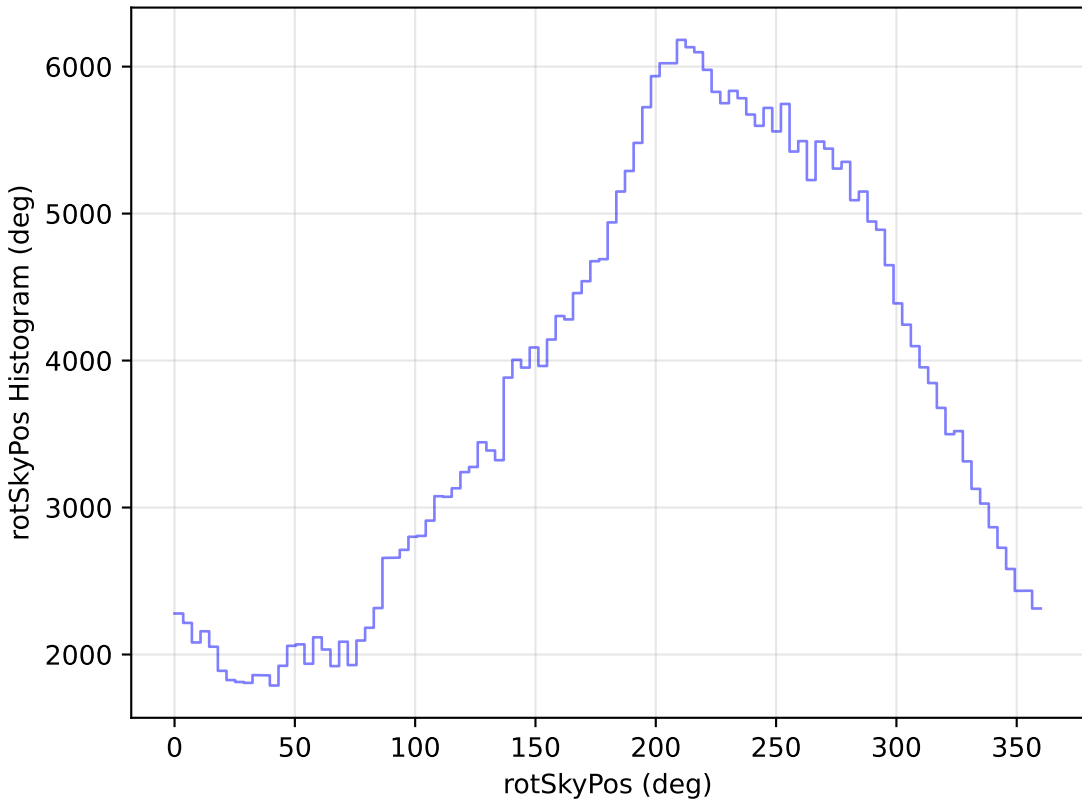
internal_u_expt30_nscale1.5v3.4_10yrs WFD y band: rotSkyPos Histogram
