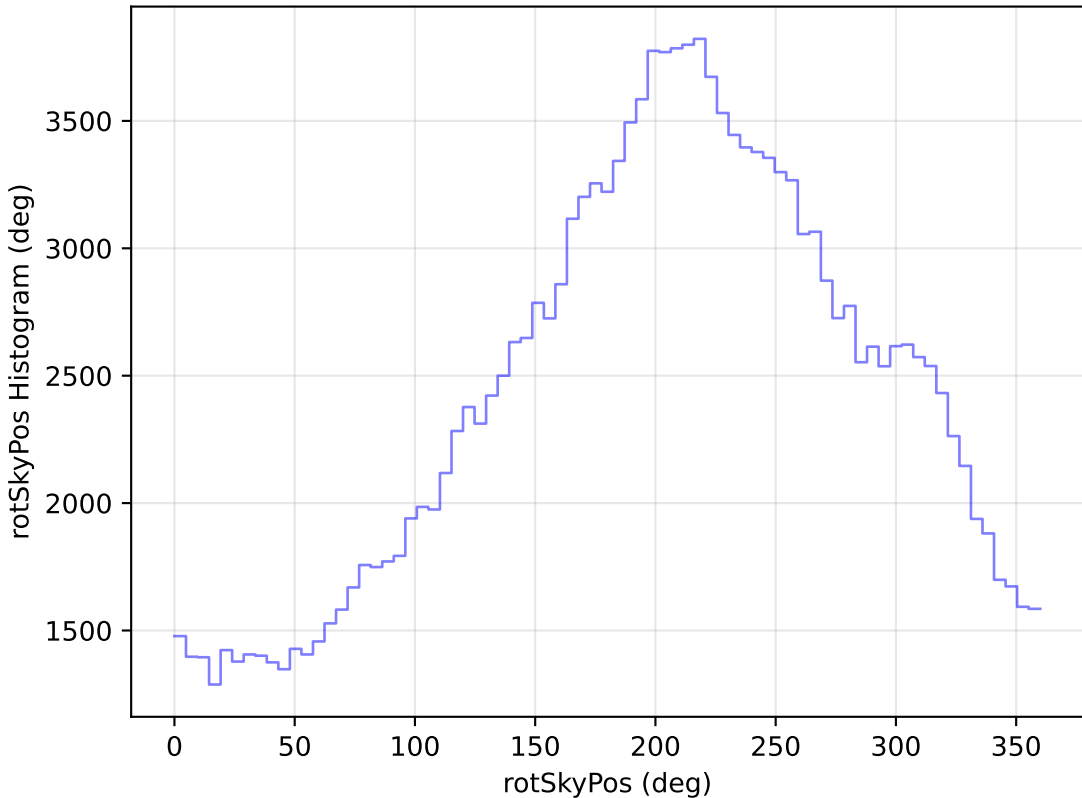
internal_u_expt30_nscale1.5v3.4_10yrs WFD u band: rotSkyPos Histogram
