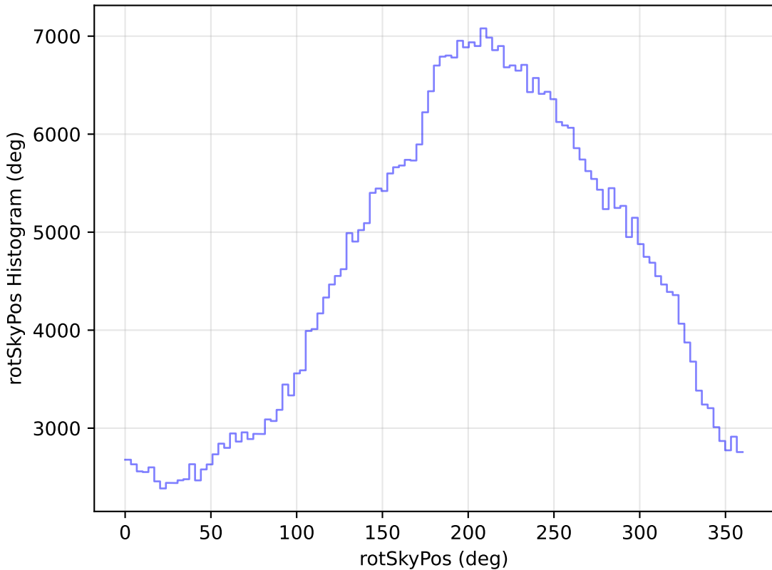
internal_u_expt30_nscale1.5v3.4_10yrs WFD i band: rotSkyPos Histogram
