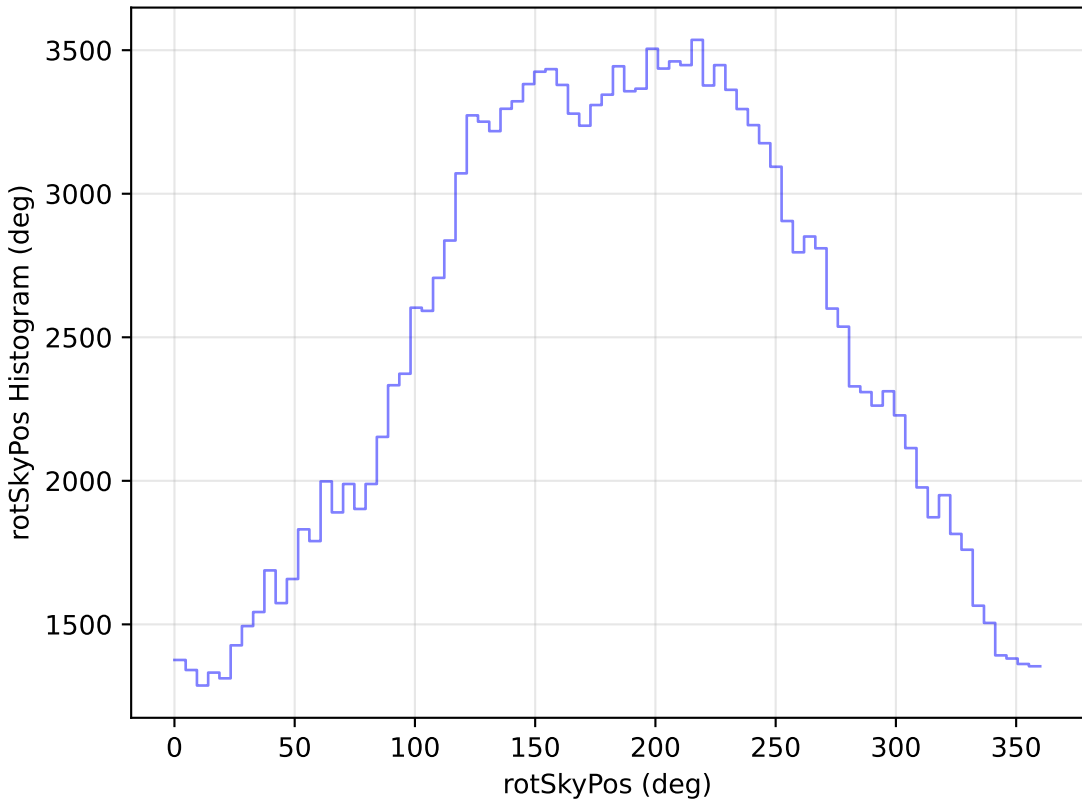
internal_u_expt30_nscale1.5v3.4_10yrs WFD g band: rotSkyPos Histogram
