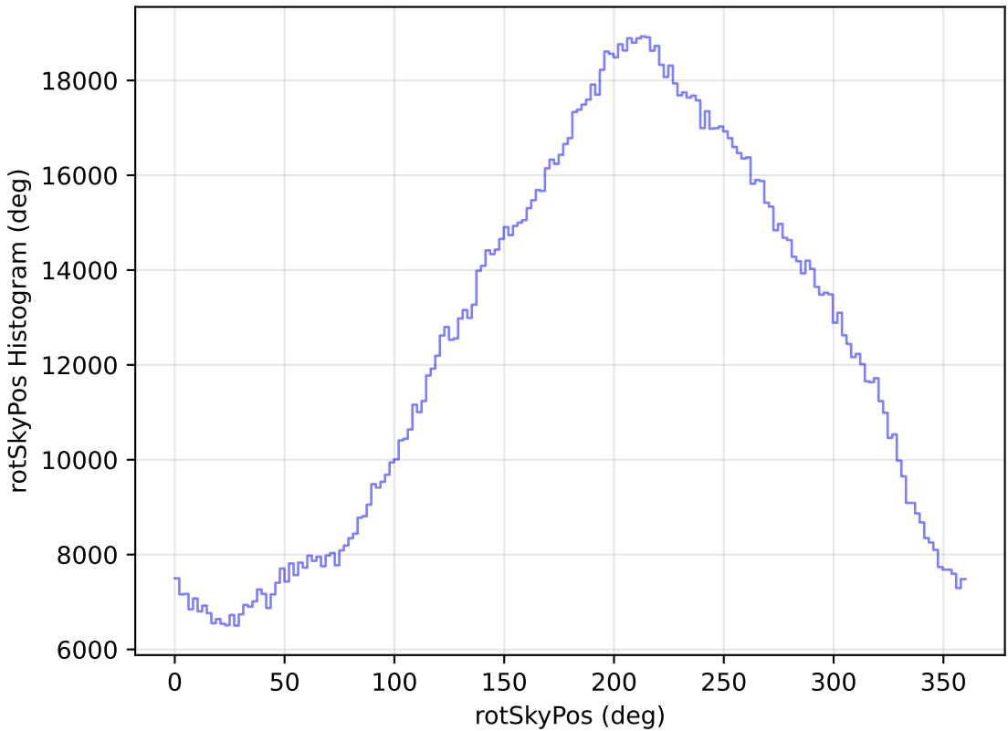
internal_u_expt30_nscale1.5v3.4_10yrs WFD all bands: rotSkyPos Histogram
