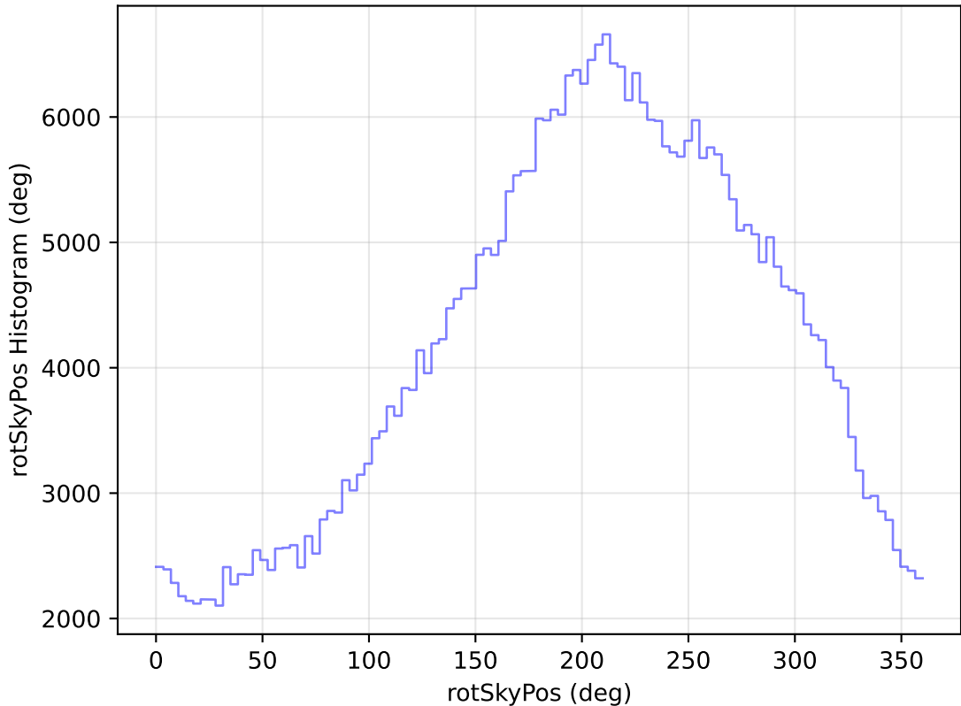
internal_u_expt30_nscale1.5v3.4_10yrs All sky z band: rotSkyPos Histogram
