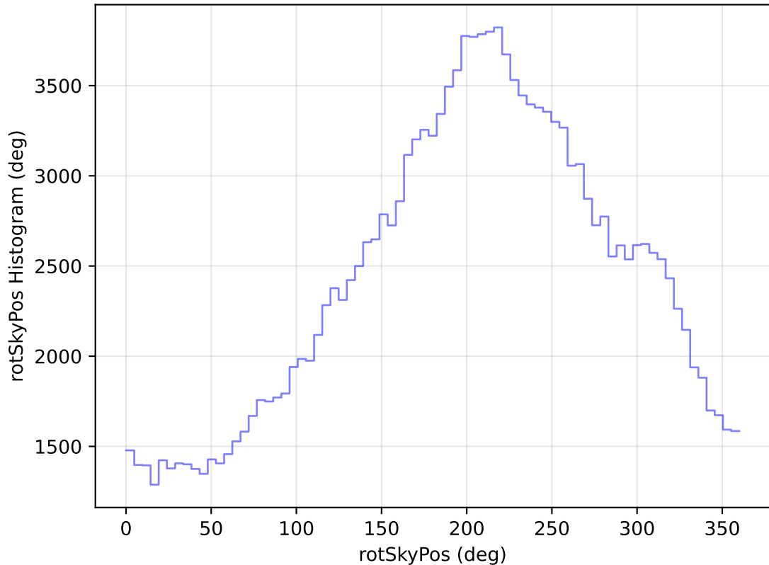
internal_u_expt30_nscale1.5v3.4_10yrs All sky u band: rotSkyPos Histogram
