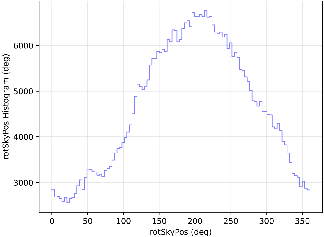
internal_u_expt30_nscale1.5v3.4_10yrs All sky r band: rotSkyPos Histogram
