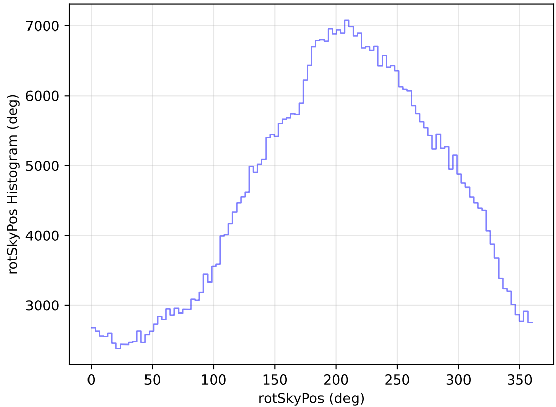
internal_u_expt30_nscale1.5v3.4_10yrs All sky i band: rotSkyPos Histogram
