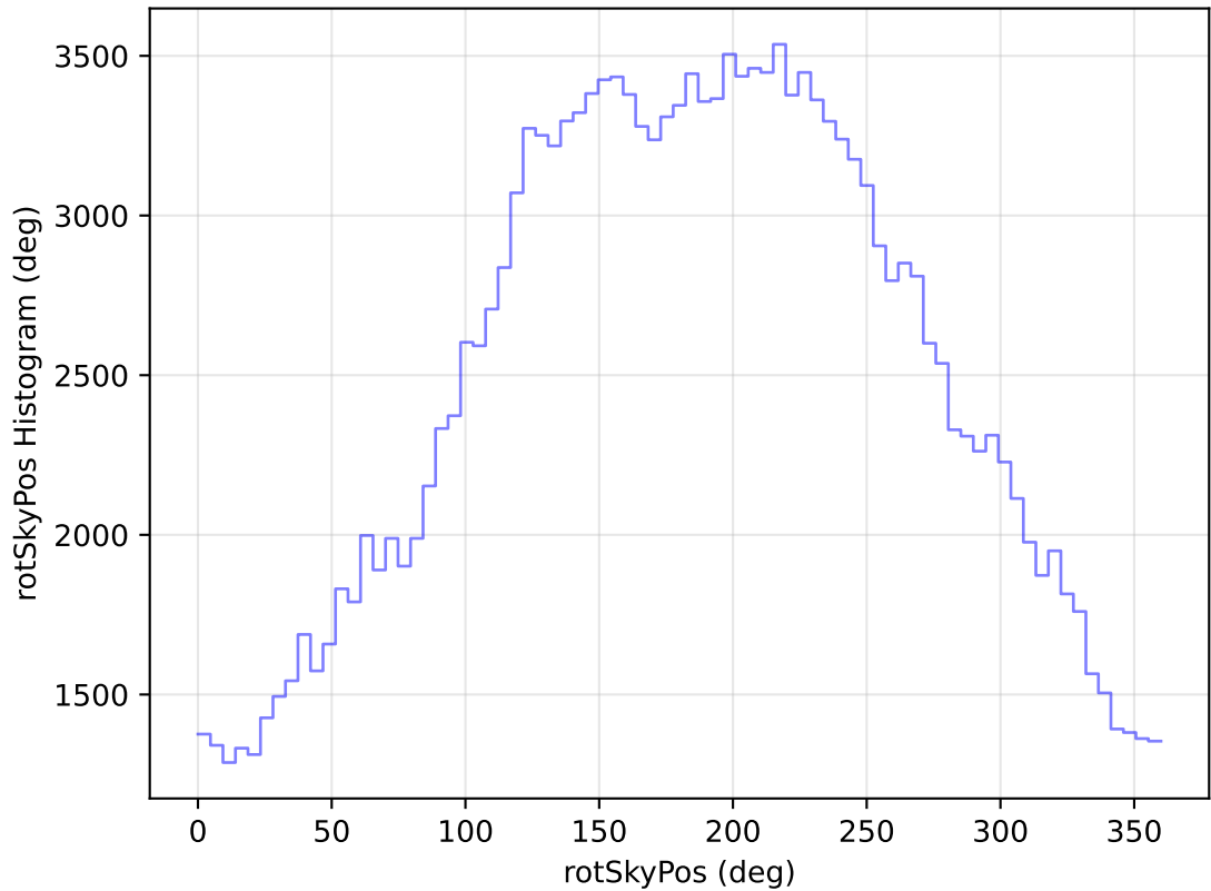
internal_u_expt30_nscale1.5v3.4_10yrs All sky g band: rotSkyPos Histogram
