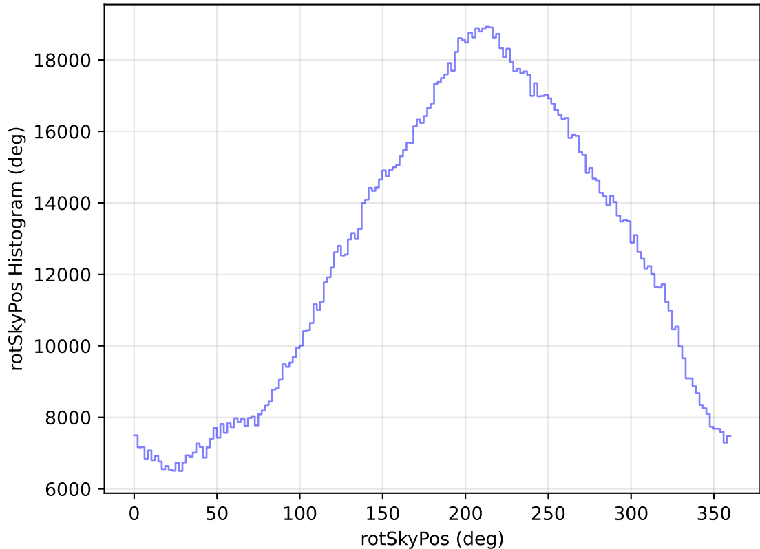
internal_u_expt30_nscale1.5v3.4_10yrs All sky all bands: rotSkyPos Histogram
