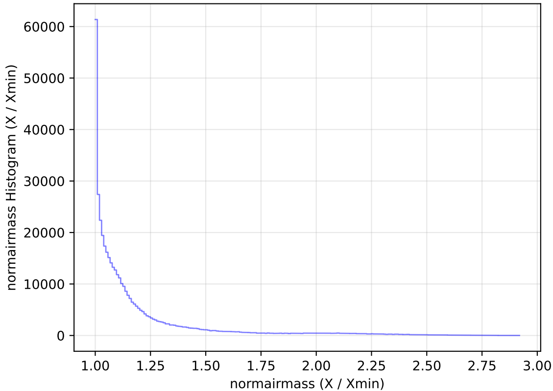
internal_u_expt30_nscale1.5v3.4_10yrs WFD z band: normairmass Histogram
