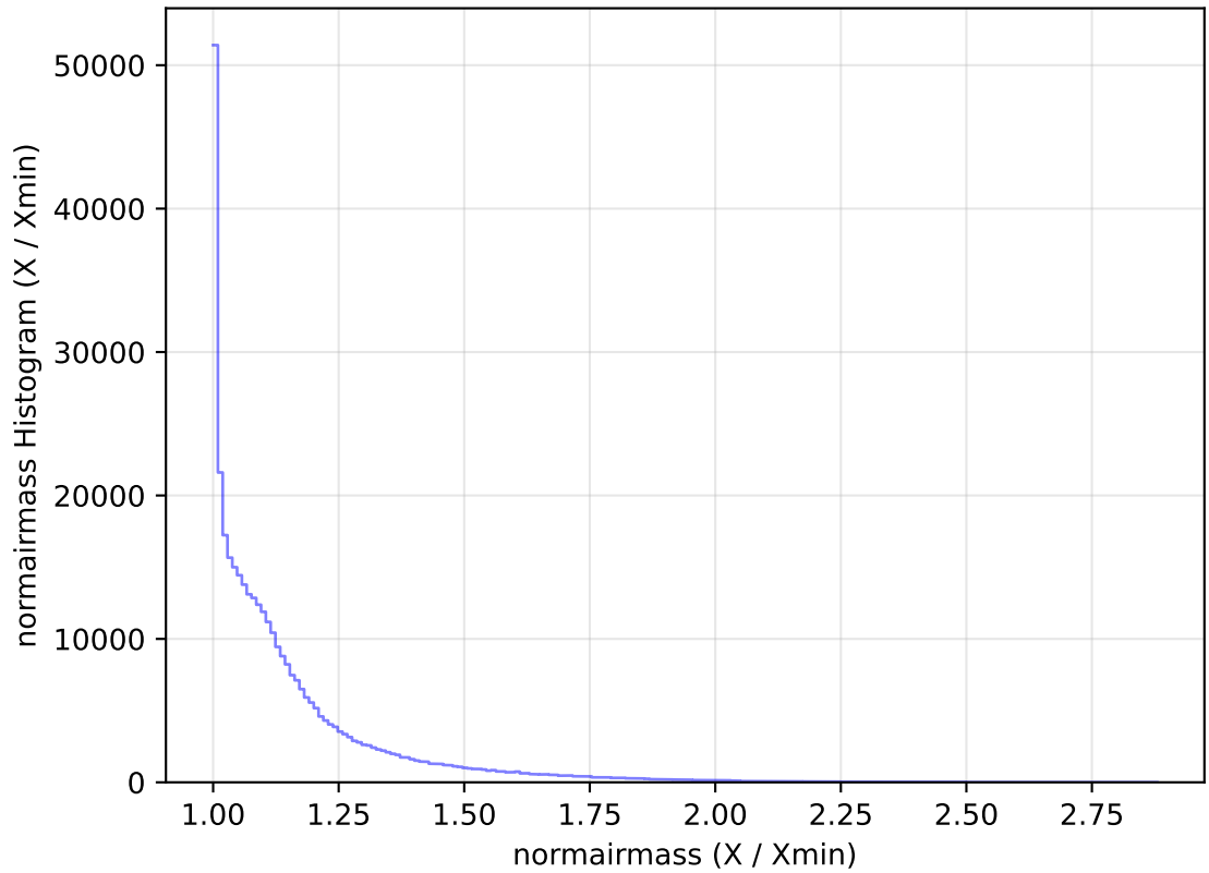
internal_u_expt30_nscale1.5v3.4_10yrs WFD y band: normairmass Histogram
