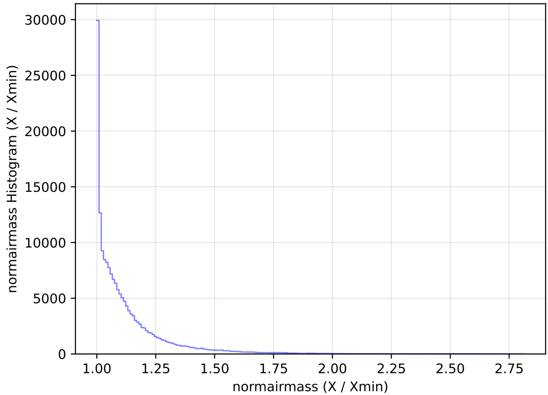
internal_u_expt30_nscale1.5v3.4_10yrs WFD u band: normairmass Histogram
