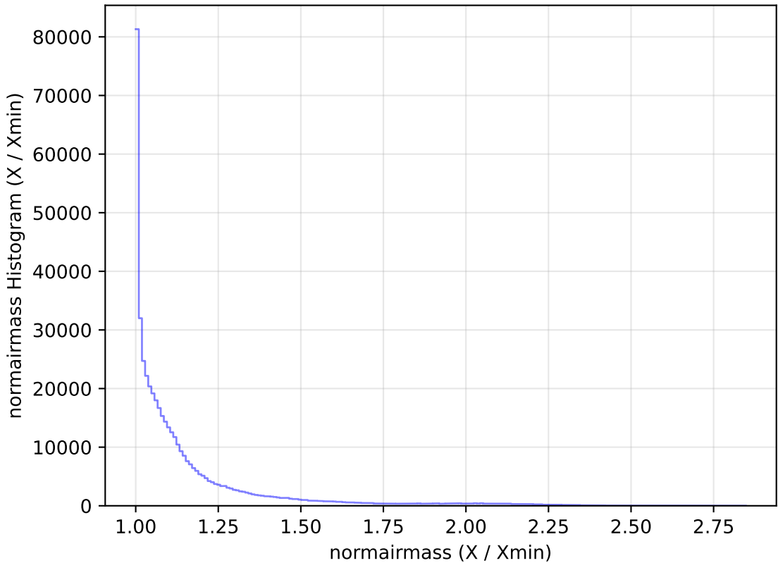
internal_u_expt30_nscale1.5v3.4_10yrs WFD r band: normairmass Histogram
