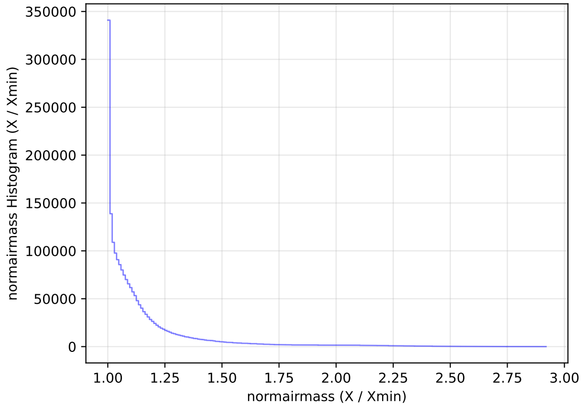
internal_u_expt30_nscale1.5v3.4_10yrs WFD all bands: normairmass Histogram
