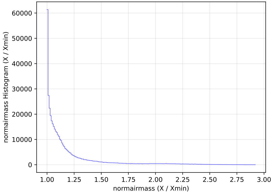
internal_u_expt30_nscale1.5v3.4_10yrs All sky z band: normairmass Histogram
