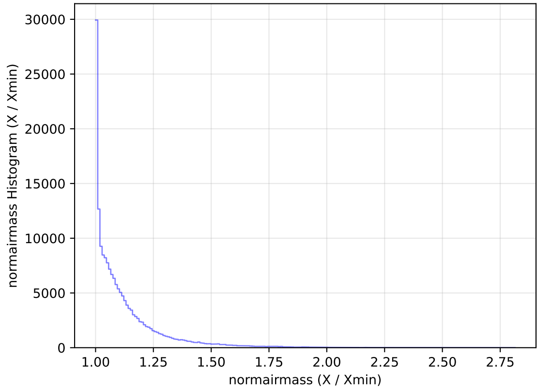
internal_u_expt30_nscale1.5v3.4_10yrs All sky u band: normairmass Histogram
