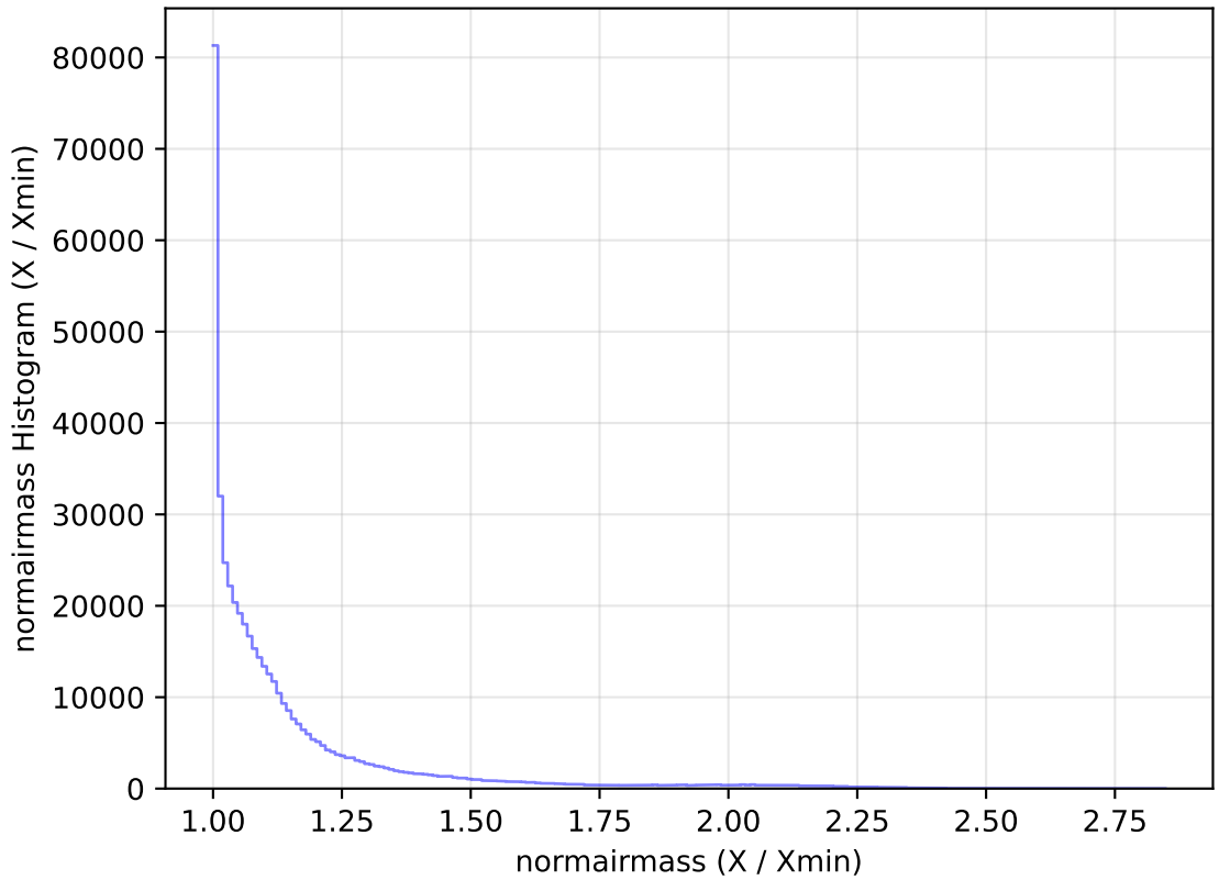
internal_u_expt30_nscale1.5v3.4_10yrs All sky r band: normairmass Histogram
