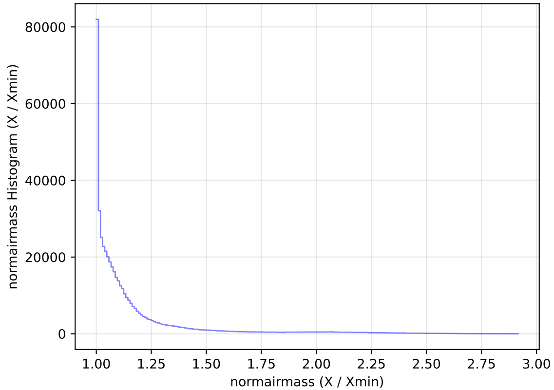
internal_u_expt30_nscale1.5v3.4_10yrs All sky i band: normairmass Histogram
