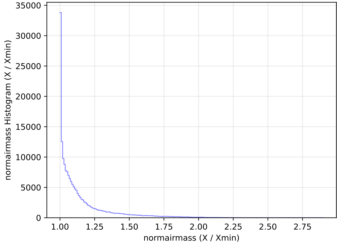
internal_u_expt30_nscale1.5v3.4_10yrs All sky g band: normairmass Histogram
