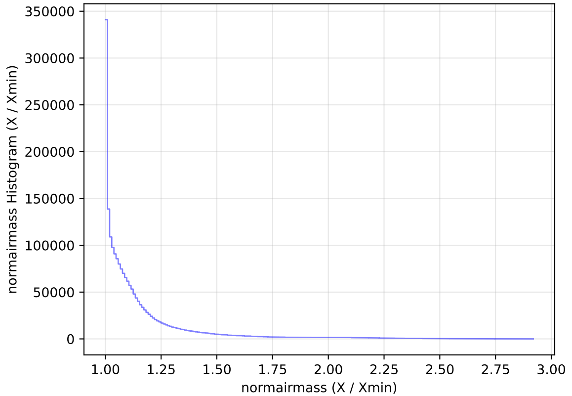
internal_u_expt30_nscale1.5v3.4_10yrs All sky all bands: normairmass Histogram
