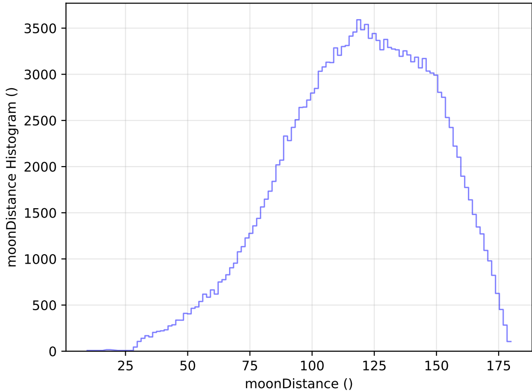
internal_u_expt30_nscale1.5v3.4_10yrs WFD u band: moonDistance Histogram
