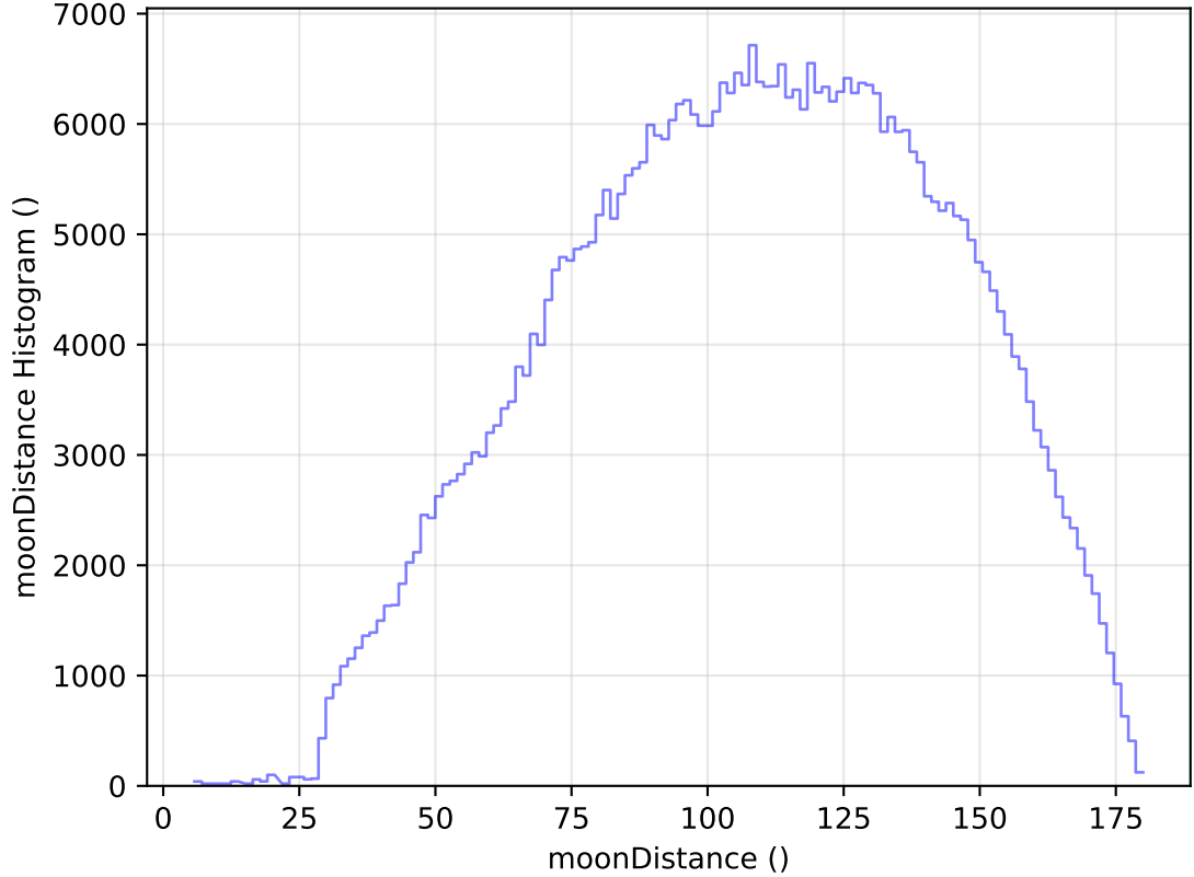
internal_u_expt30_nscale1.5v3.4_10yrs WFD r band: moonDistance Histogram
