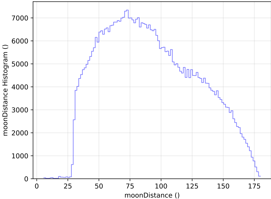
internal_u_expt30_nscale1.5v3.4_10yrs WFD i band: moonDistance Histogram
