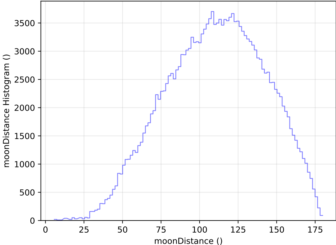
internal_u_expt30_nscale1.5v3.4_10yrs WFD g band: moonDistance Histogram
