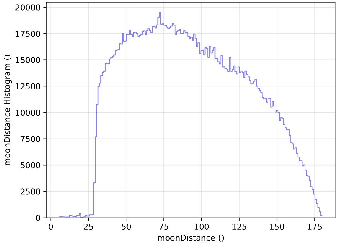
internal_u_expt30_nscale1.5v3.4_10yrs WFD all bands: moonDistance Histogram
